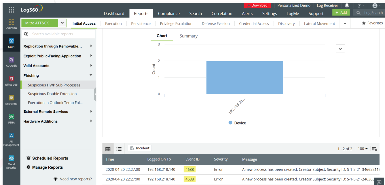
Figure 10-1: Detecting initial access from the phishing technique with ATT&CK reports in Log360
