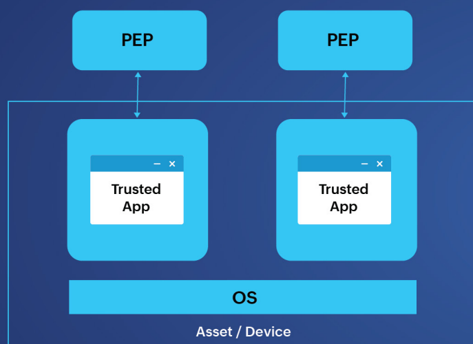
Figure 8: Application sandboxing.
