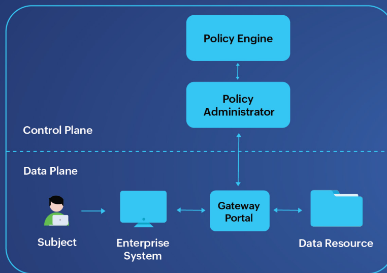
Figure 7: Resource portal-based model.
